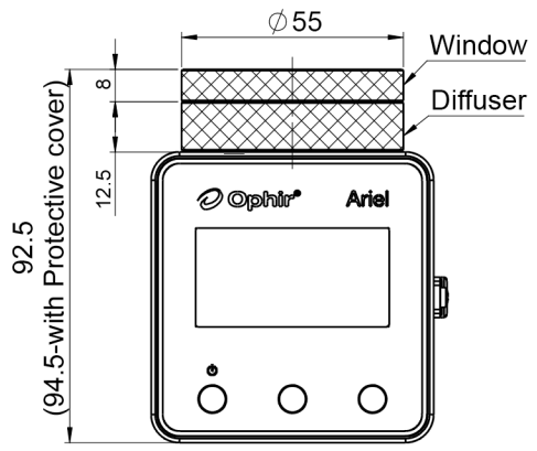
Ariel-V2 Mounted With Diffuser & Window
