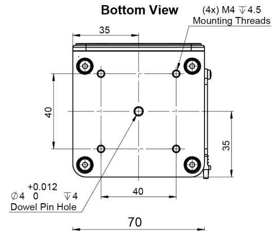
Ariel-V2 (More Detail View)
